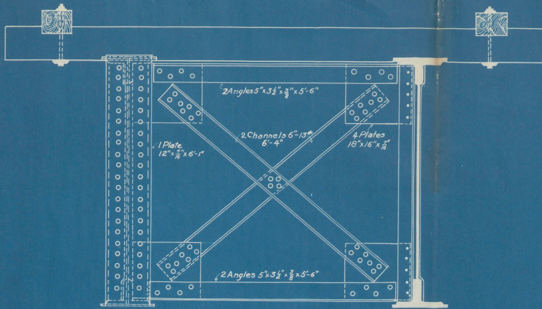
END CROSS FRAME
