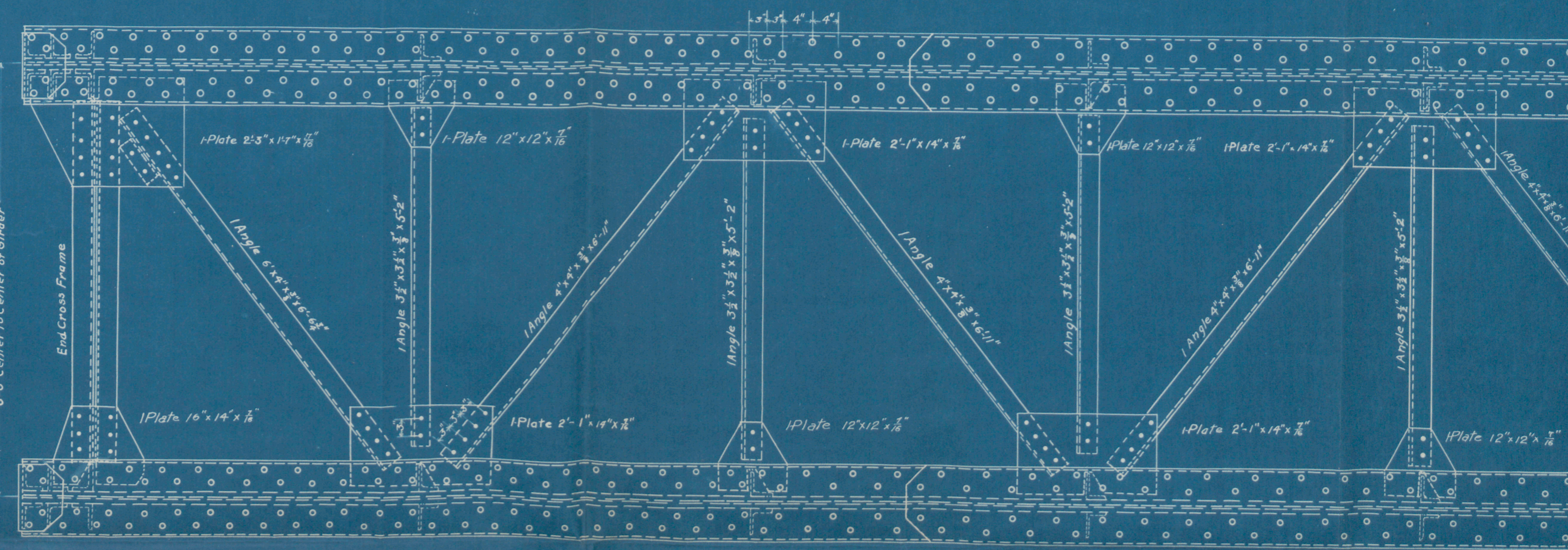
TOP LATERAL BRACING
