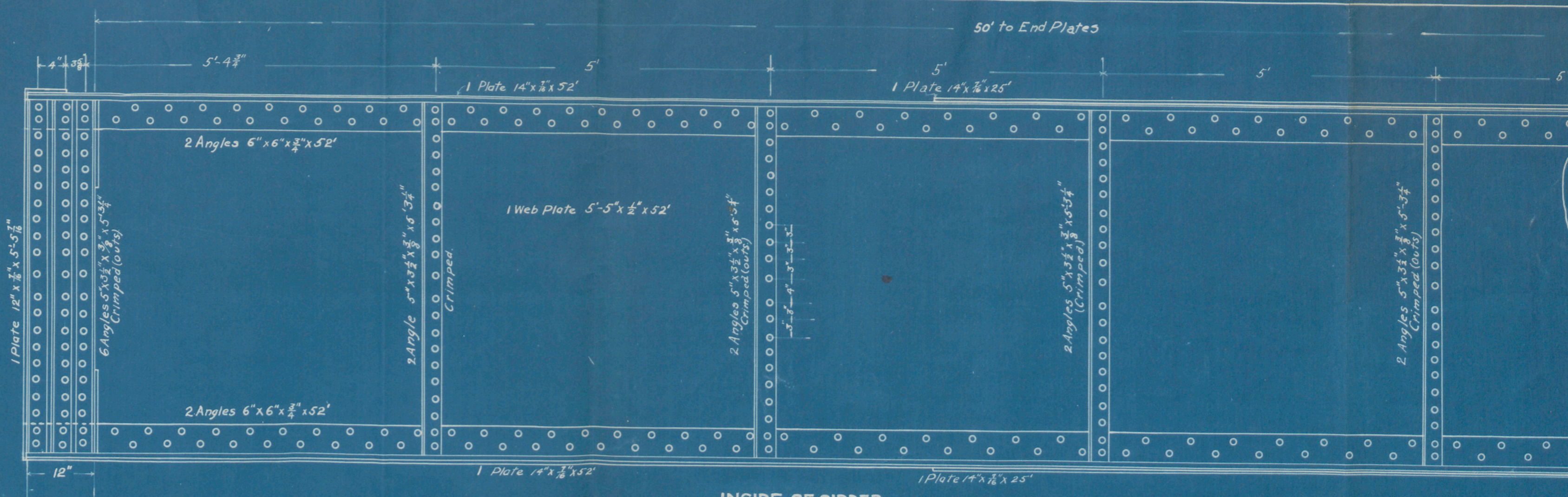
INSIDE OF GIRDER
