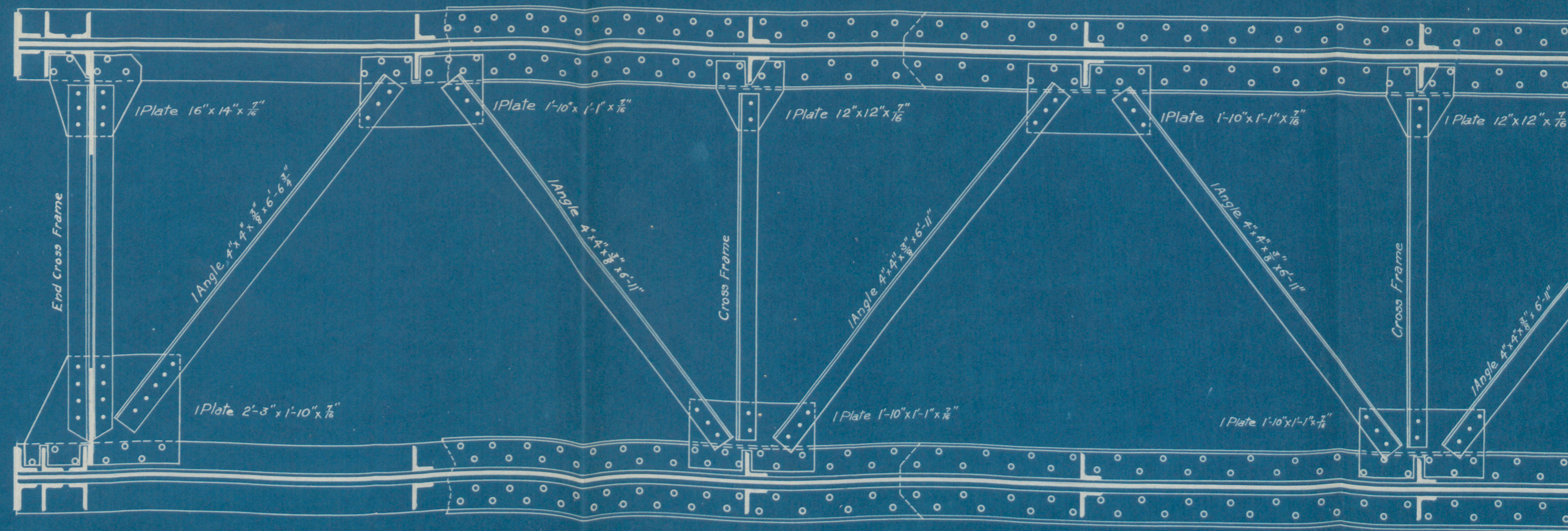
BOTTOM LATERAL BRACING
