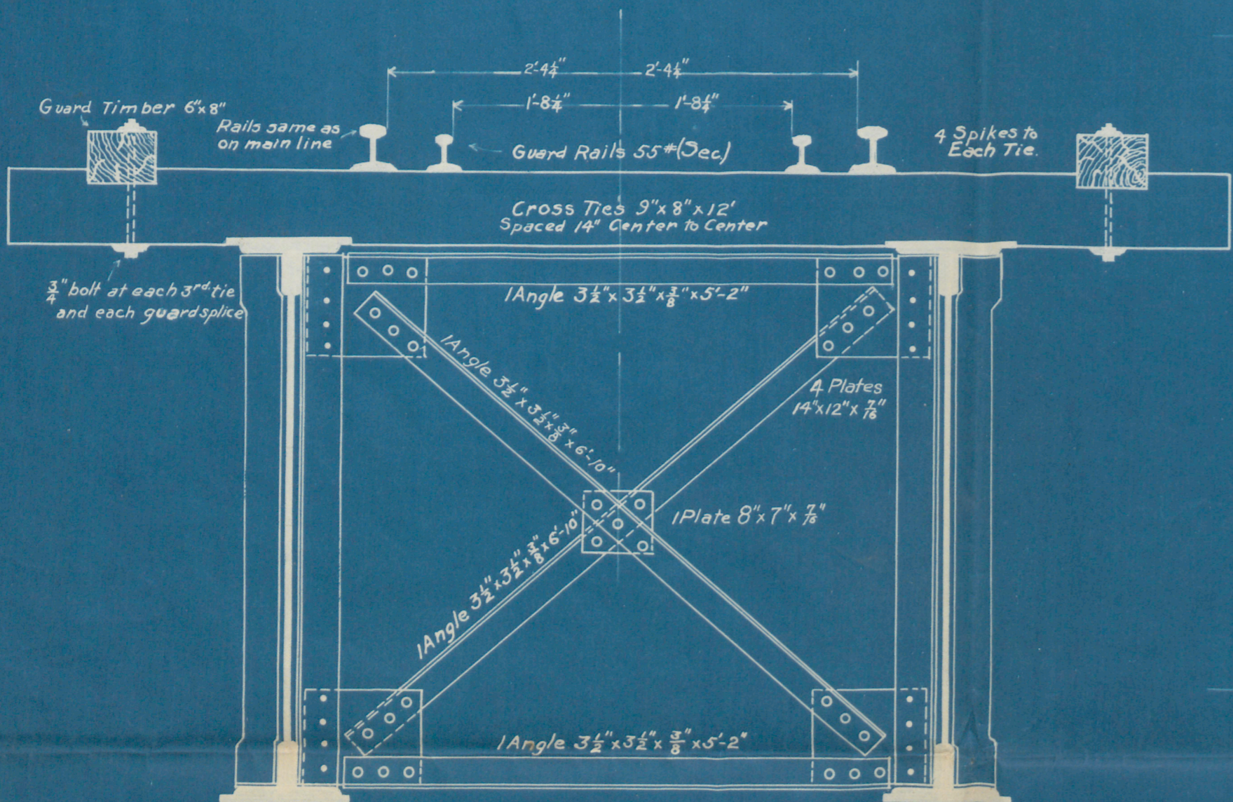
INTERMEDIATE CROSS FRAME
